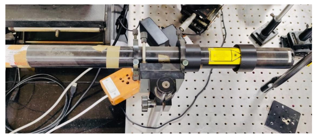
He-Ne LASER
